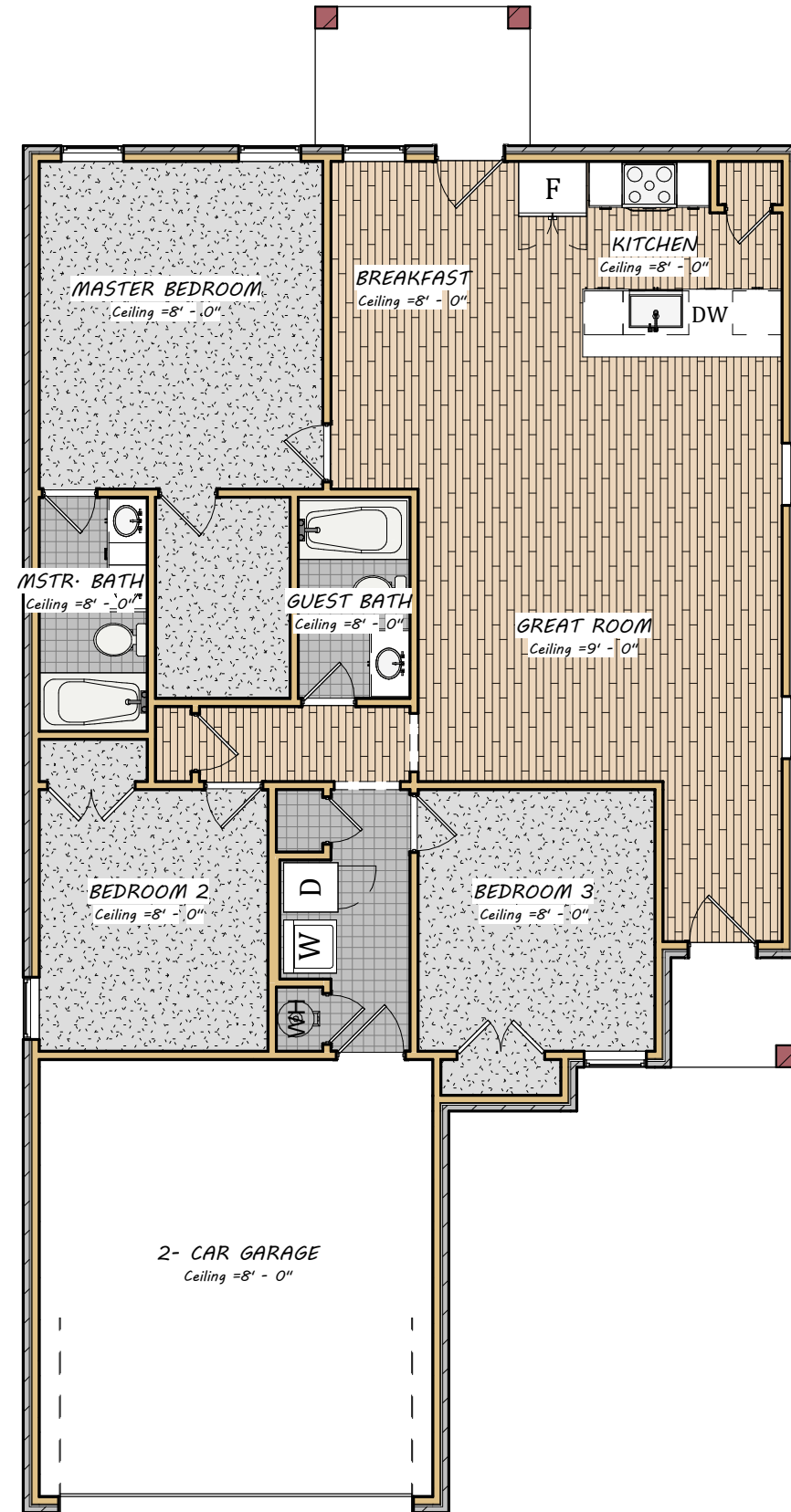
① Level 1 Layout 1/8" = 1'-0"
